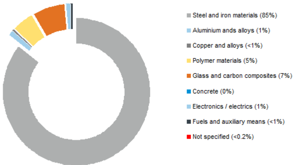
Figure 6: Material breakdown of 100MW power plant of V117-3.3 MW turbines (% mass)
