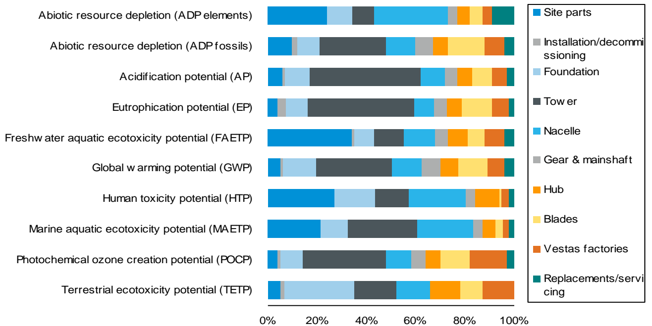
Figure 7: Production and use-phase environmental impacts of V117-3.3 MW
