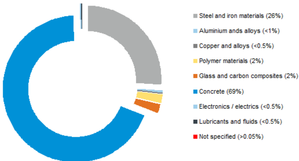
Figure 6: Material breakdown of 100MW power plant of V117-3.3 MW turbines (% mass)
